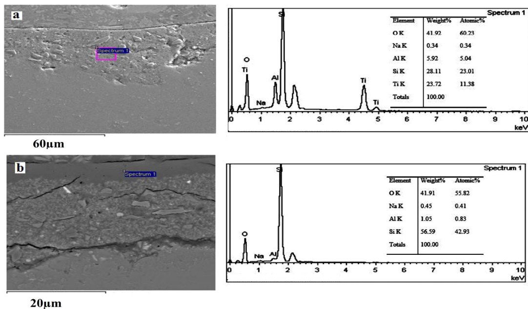
Fig. 2 SEM image and EDAX of the cross-section of the sprayed coating on aluminum substrate a Basecoat (M3), b Top coat (M3)
