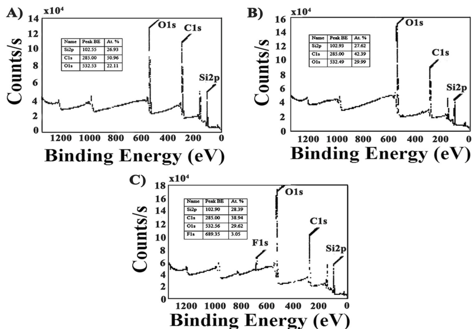
Fig. 4 XPS spectra of the top surface of a M1, b M2 and c M3
