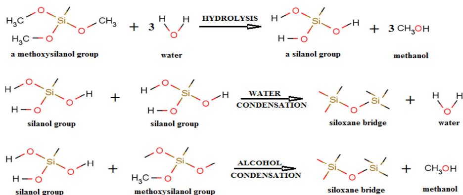
Scheme 2 The sol-gel process
