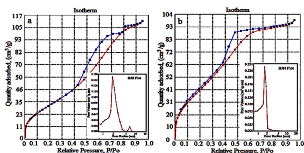
Fig. 1 N 2 adsorption-desorption isotherms and pore size distribution of the (a) base and (b) top coat (M3)
