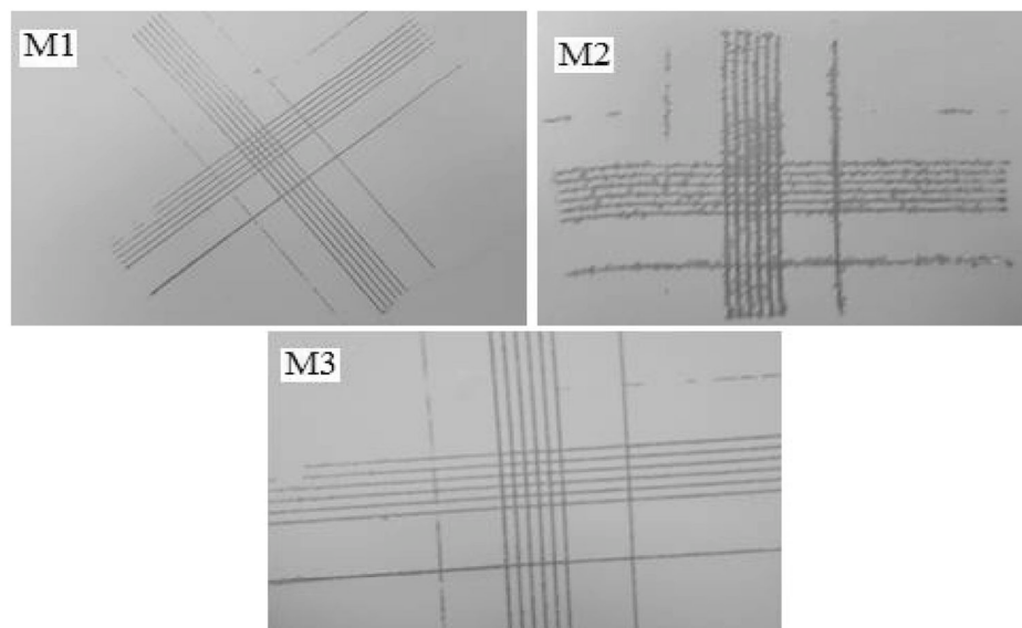
Fig. 6 Cross-cut results of sol-gel-coated Al substrates
