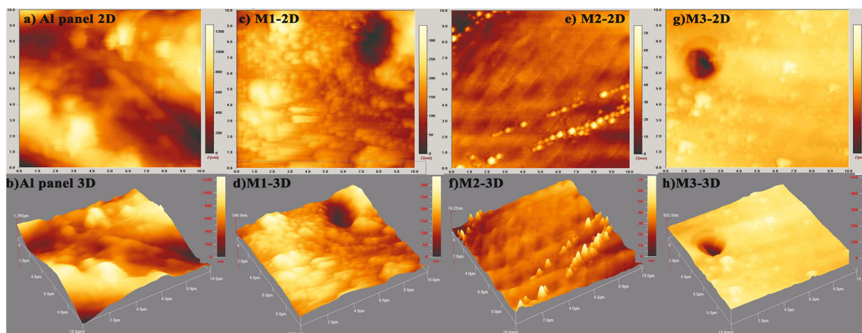
Fig. 3 AFM images of sandblasted aluminum panels, M1, M2 and M3
